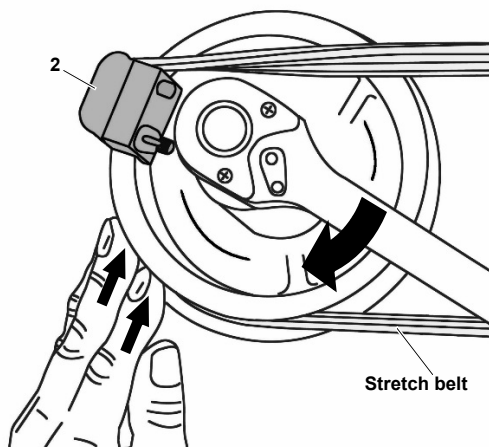
Fig. 5: Installing the stretch belt with the aid of the belt installation tool.
